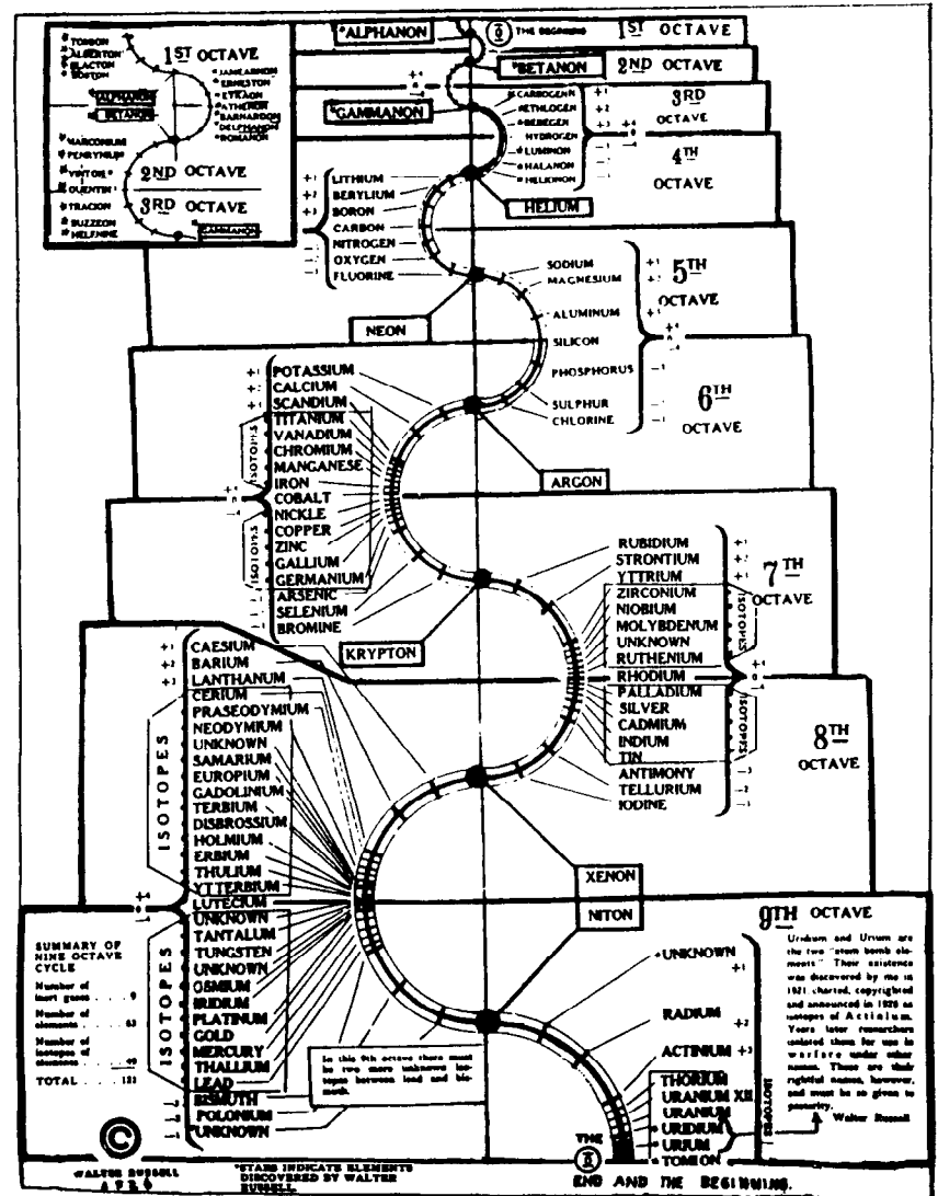
FIG. 68 The Russell Periodic Chart of the Elements, No. 1
